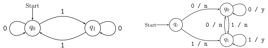
Fig. 8. (left) Finite automaton for parity, (right) Example Mealy machine
