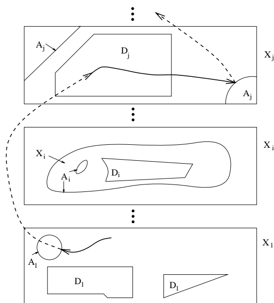
Fig. 12. Example dynamics of an HDS
