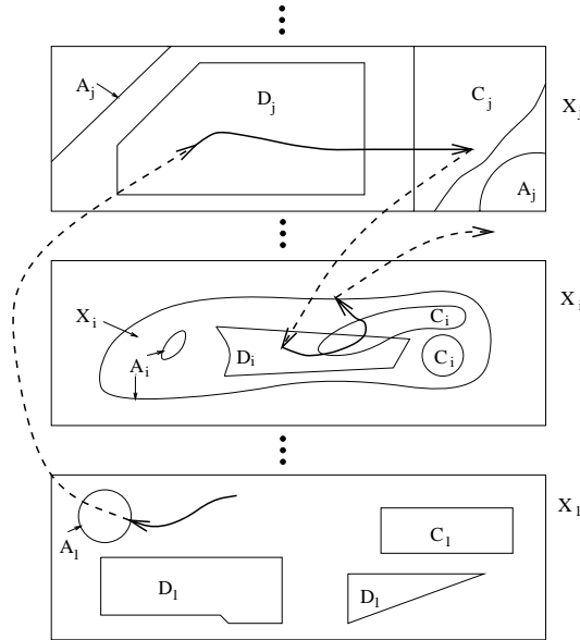
Fig. 16. Example dynamics of a CHDS
