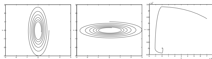
Fig. 7. Trajectories for (left) A_1x , (center) A_2x , and (right) a switched linear system
